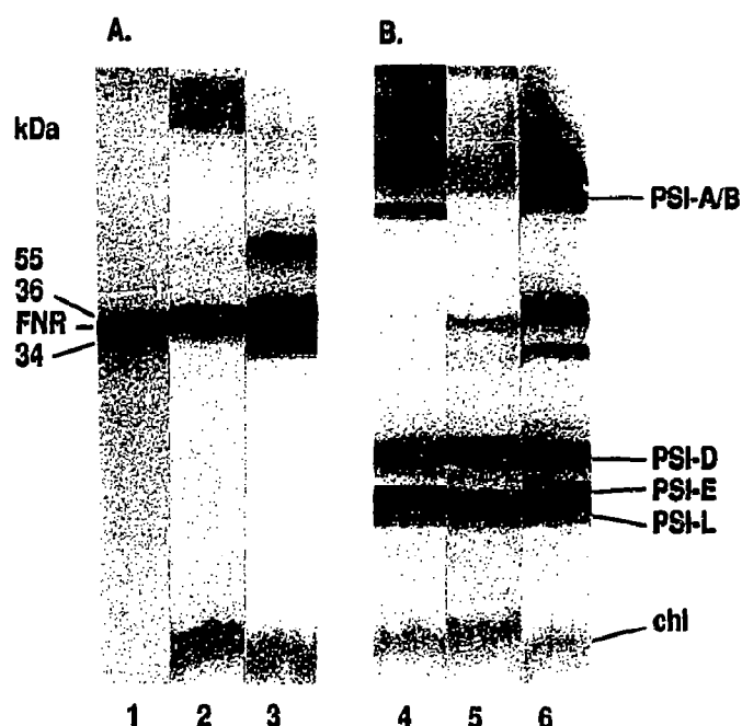
Fig. 2. Western blot analysis of cross-linking of DM-PS I with DTSSP and EDC. (Lanes 1 and 4) DM-PS I; (lanes 2 and 5) DM-PS I cross-linked with EDC; (lanes 3 and 6) DM-PS I cross-linked with DTSSP. Lanes 1-3 were incubated with antibodies against FNR. Lanes 4-6 were incubated with antibodies raised against TX-PS I. The electrophoresis was performed without reductant in the sample buffer resulting in diffuse bands on the Western blot.
